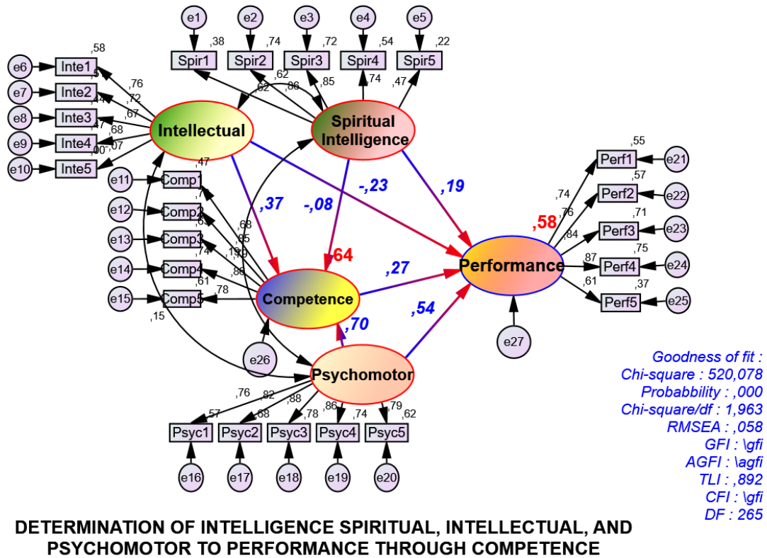
Figure 2. Full Model SEM
