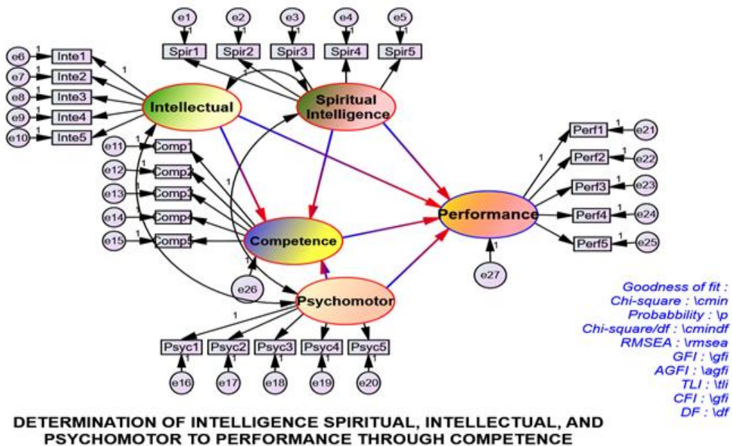
Figure 1. Conceptual Model Research
